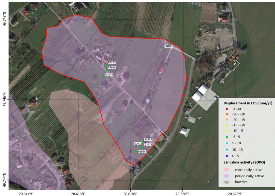
Fig. 3 Point displacement in LOS values (descending dataset) and landslides activity from SOPO database
