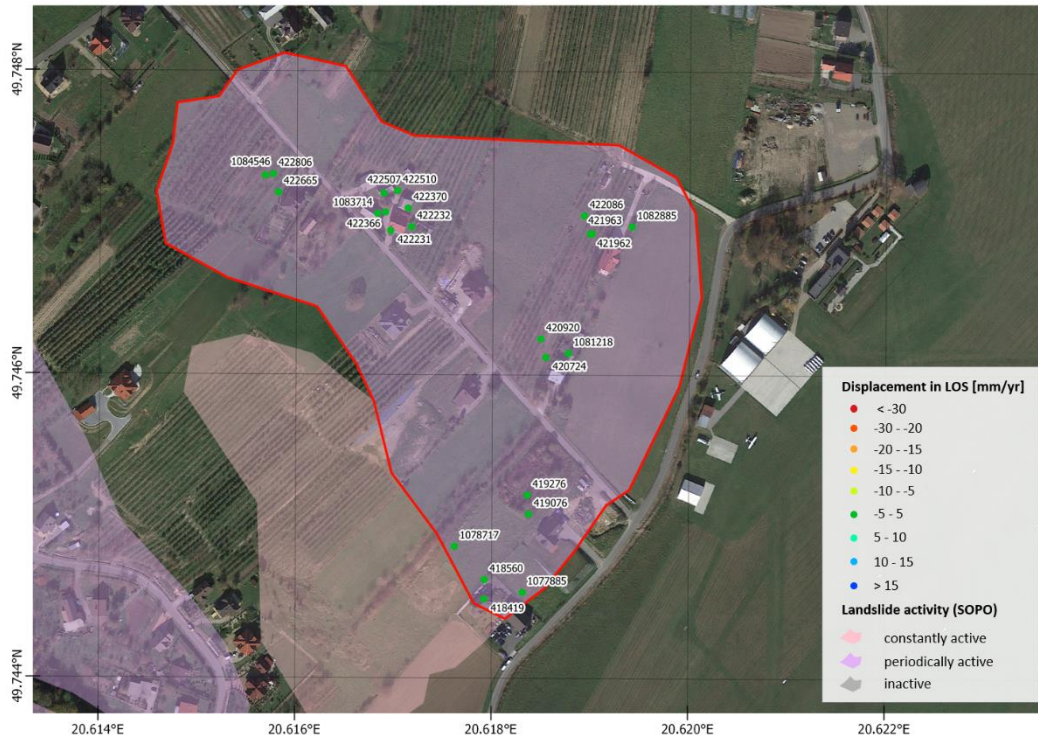
Fig. 2 Point displacement in LOS values (ascending dataset) and landslides activity from SOPO database
